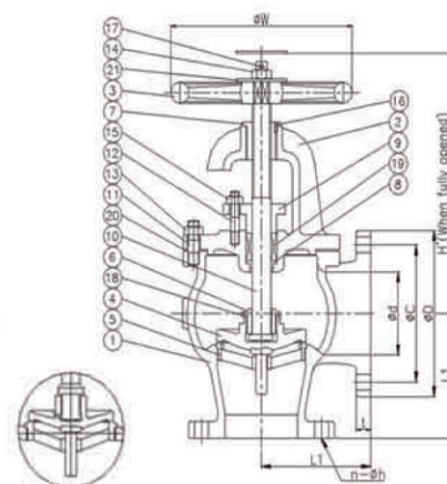
Screw-down check valve
