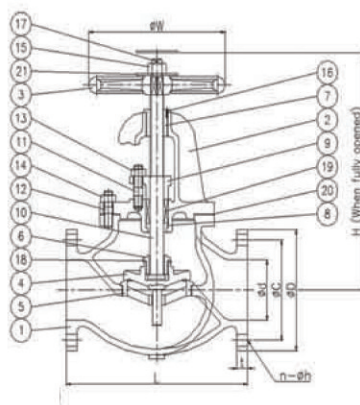
GLOBE VALVE
